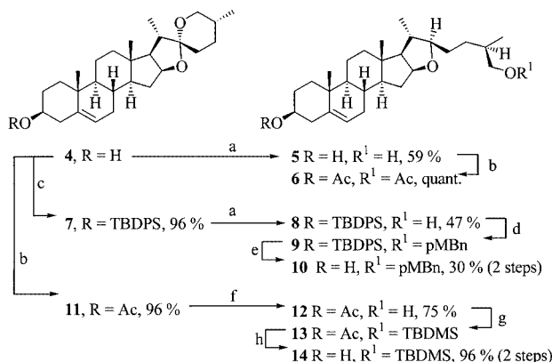
Scheme 1. a: LiAlH 4 /AlCl 3 /Et 2 O; b: Ac 2 O, pyridine; c: TBDPSCl, imidazole, DMF; d: pMBnCl, NaH, DMF; e: TBAF, THF; f: AcOH, NaBH 3 CN; g: TBDMSCl, pyridine; h: NaOMe, MeOH
