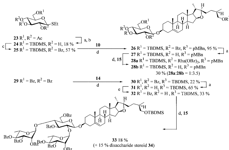
Scheme 4. a: NaOMe/MeOH; b: TBDMSCl, NEt 3 , DMAP, DMF, 48 h, room temp.; c: benzoyl chloride, pyridine, DMAP, 0 °C → room temp., 5 d; d: DMTST, Et 2 O, 4-Å mol. sieves, argon or N 2 ; e: 1-BBTZ, NEt 3 , CH 2 Cl 2
